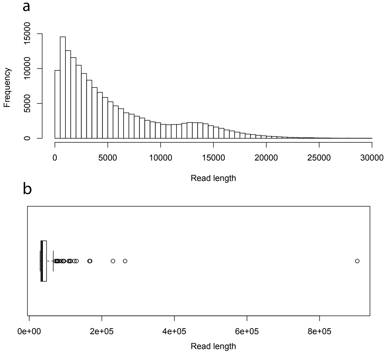
Figure S1. Size distribution of the Nanopore sequencing data of the total DNA. a. histogram of the size of the 162,123 reads \leq 30\text{Kb} and b. box plot of the size of the 122 reads > 30\text{Kb} .
